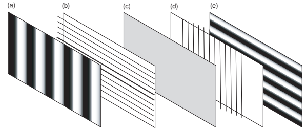
Fig. 3. Layers in a LCD
