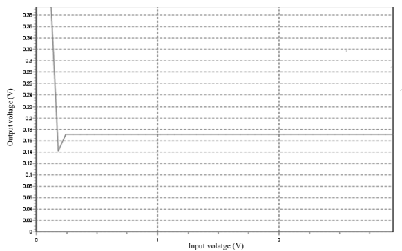
Fig. 8. Example 1 of LC response
