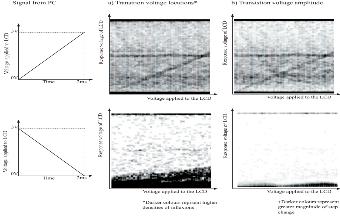
Fig. 12. Map of transition voltages discovered by evolution in the LCD when presented with a voltage ramp
