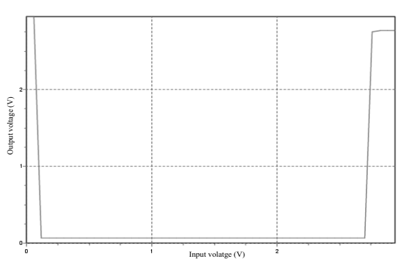
Fig. 9. Example 2 of LC response
