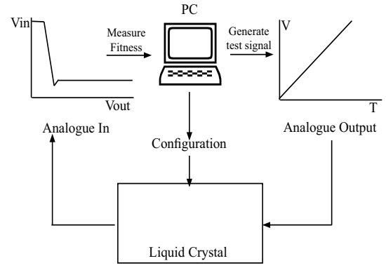
Fig. 2. Equipment configuration
