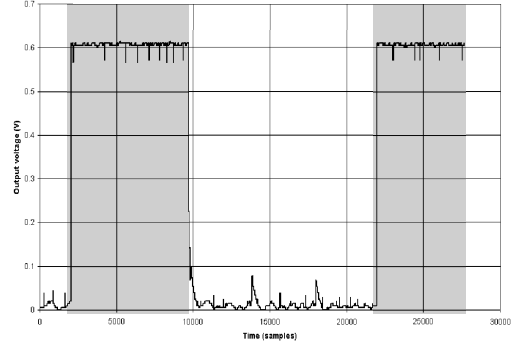
Fig. 13. Tone discriminator response. Dark areas indicate 5kHz input, light 100Hz
