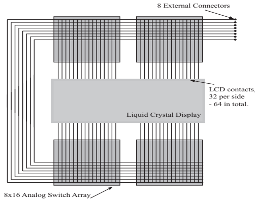
Fig. 5. Schematic of LCEM
