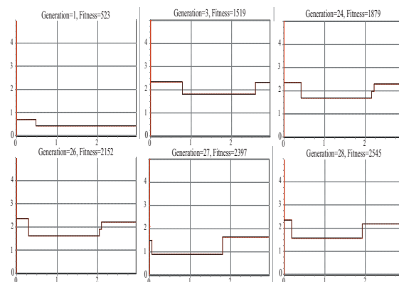
Fig. 11. Sequence showing evolution of response at 2V (output vs. input voltage)
