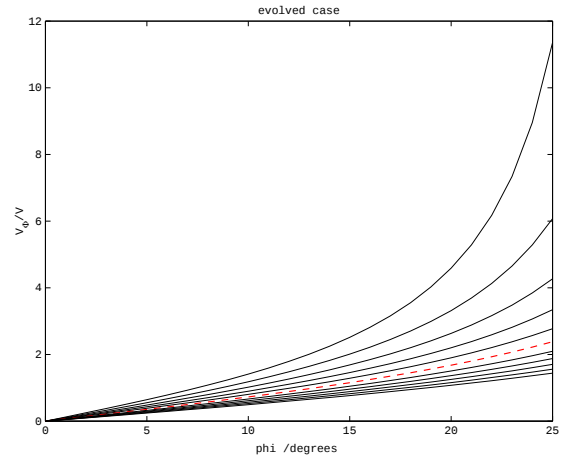
Figure 12: V_\phi against \phi with different \alpha values using the evolved solution
