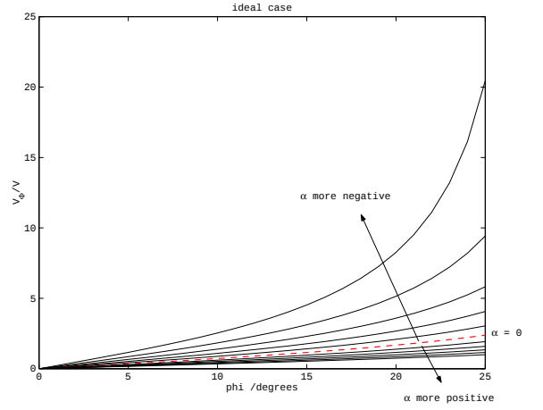
Figure 11: V_\phi against \phi with different \alpha values using the original solution
