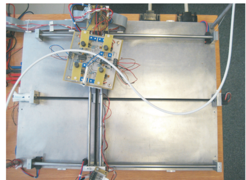
Figure 14: Top View of Shaky Hand
