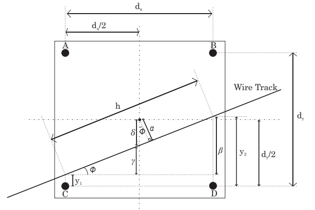
Figure 8: Plate model to create CGP input sets
