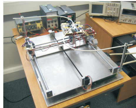
Figure 13: General View of Shaky Hand
