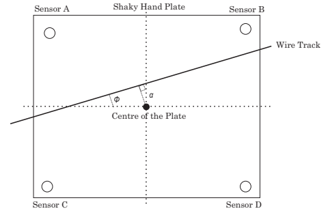
Figure 4: Four sensors on the Shaky Hand plate and the offset terms
