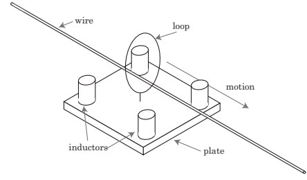
Figure 3: The Shaky Hand game pickup plate
