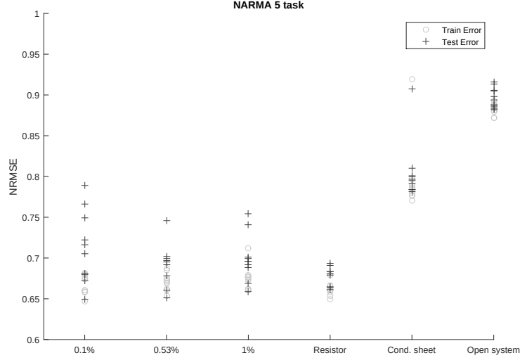
Fig.4: NARMA-5 plot of train and test error of 10 runs across all materials (lower error is better fitness). All test subjects outperform the open system; all with the exception of some 0.1% concentration runs outperform the conductive sheet in all runs.
